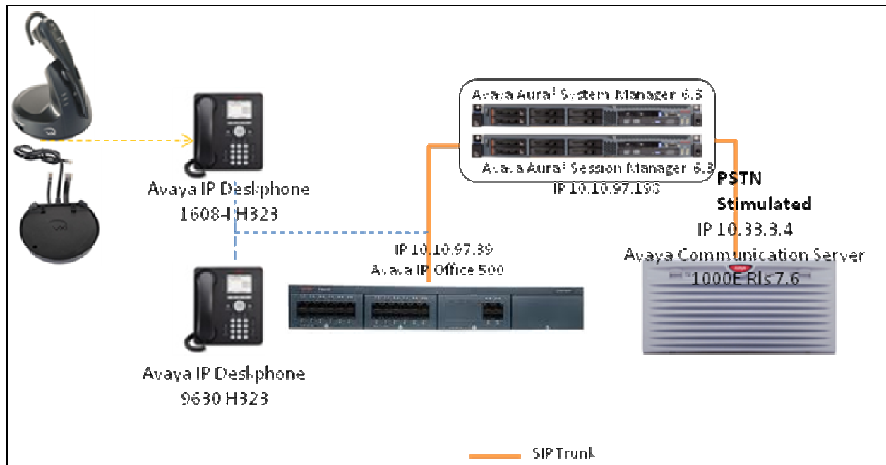
Figure 1: Test Configuration
