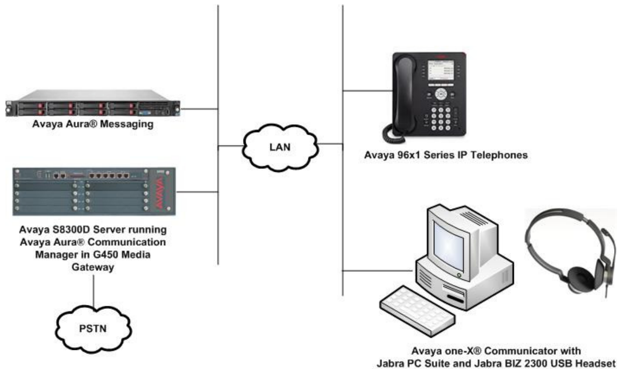
Figure 1: Test Configuration with Avaya one-X® Communicator and Jabra PC Suite and Jabra BIZ 2300 USB Headset
