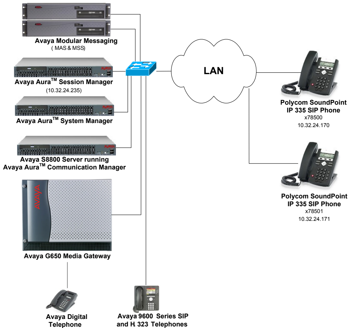
Figure 1: Avaya SIP Network with Polycom SoundPoint IP 335 SIP Phones
