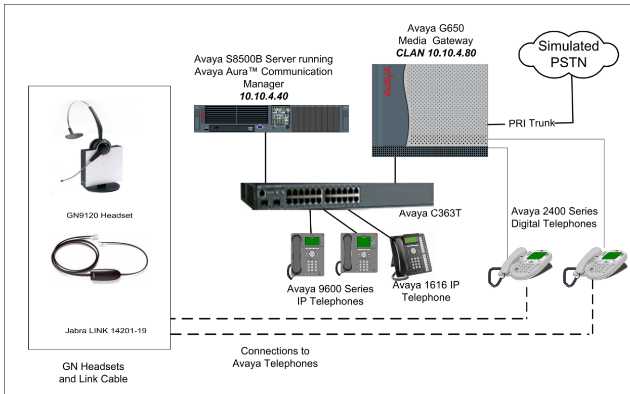
Figure 1: Network Topology
