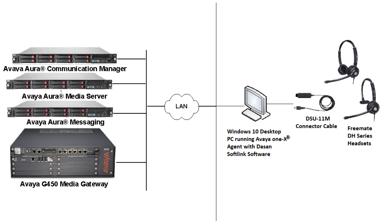
Figure 1: Test Configuration
