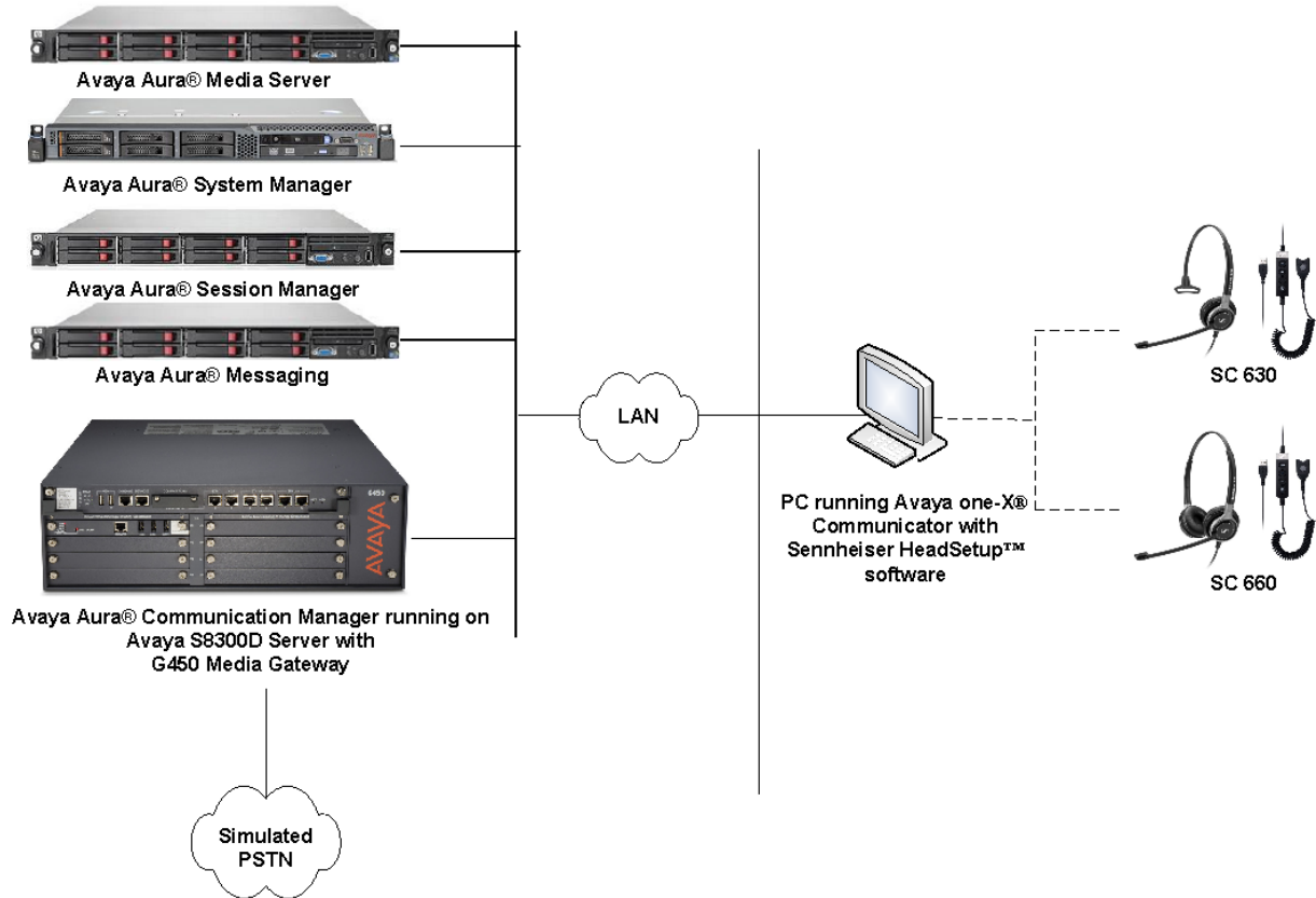
Figure 1: Test Configuration
