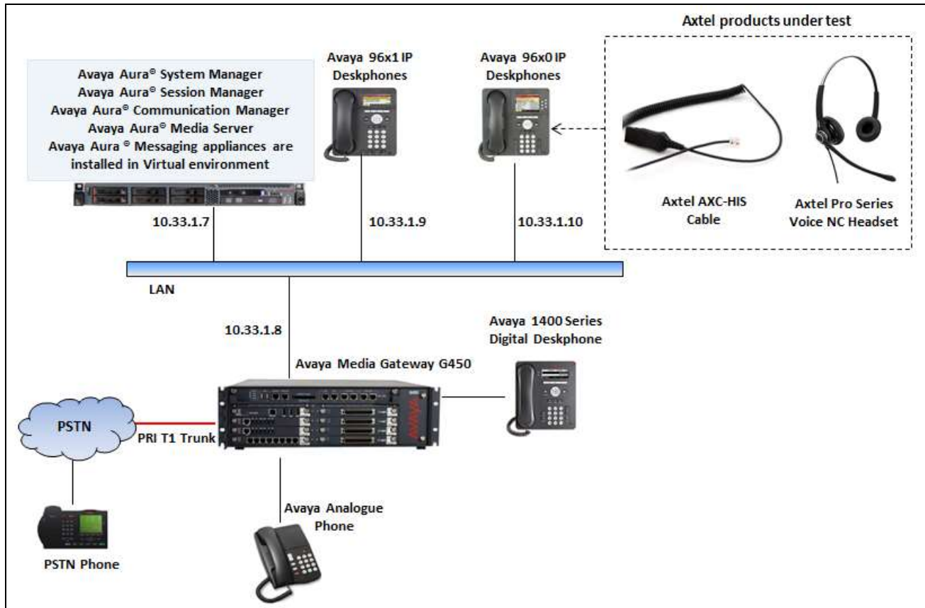
Figure 1: Avaya 96x0 Series IP Deskphones with Axtel AXC-HIS Cable & Axtel Pro Series Mono/Duo NC Headset
