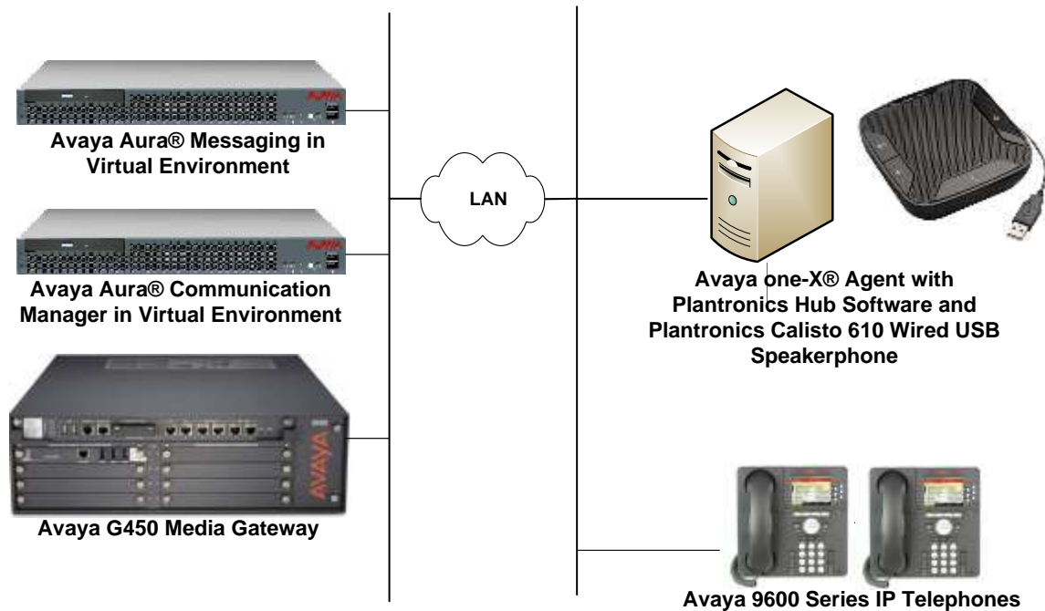
Figure 1: Avaya one-X Agent with Plantronics Hub Software and Plantronics Calisto 610 Wired USB Speakerphone
