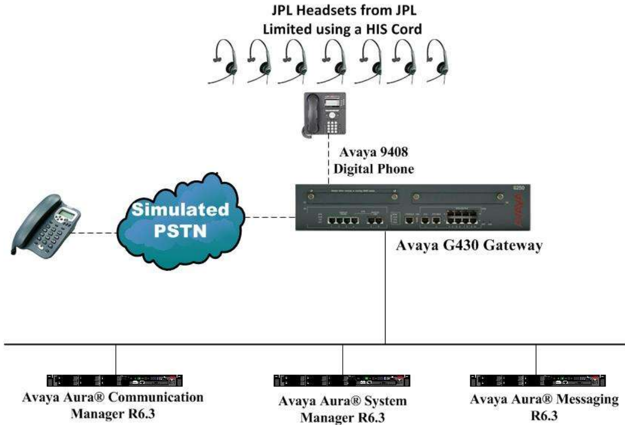
Figure 1: Network Solution of the JPL Headsets connecting to Avaya 9400 Series Digital Telephones using a HIS cord
