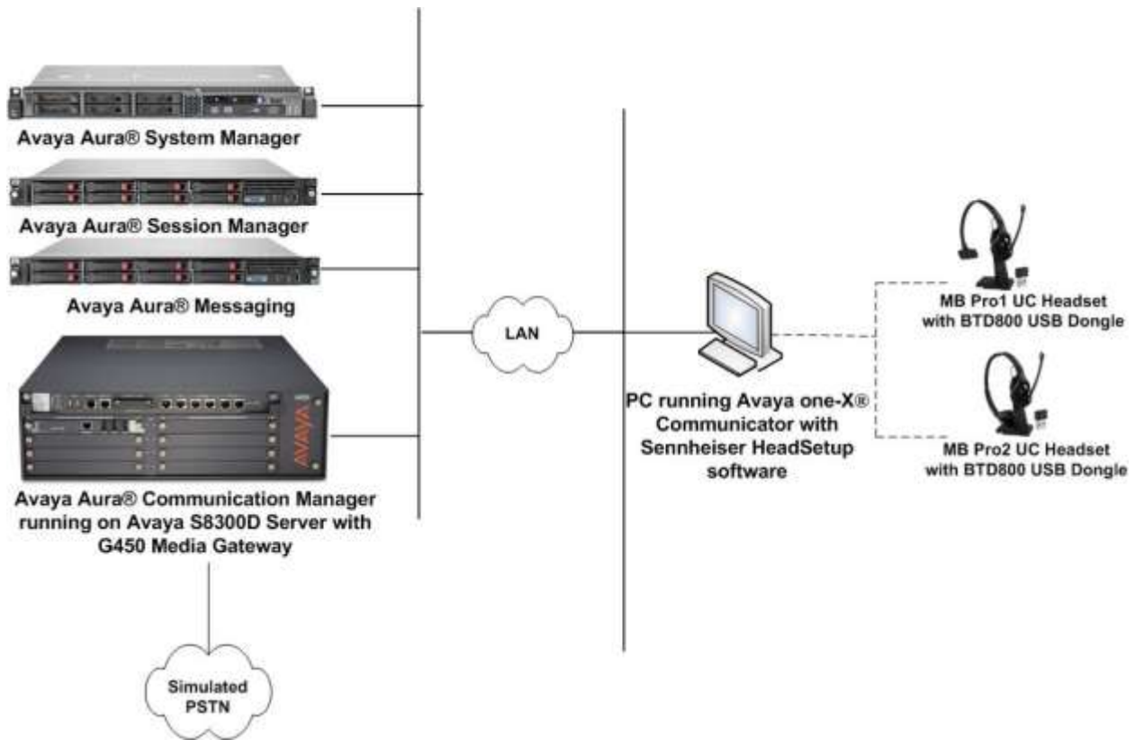
Figure 1: Test Configuration
