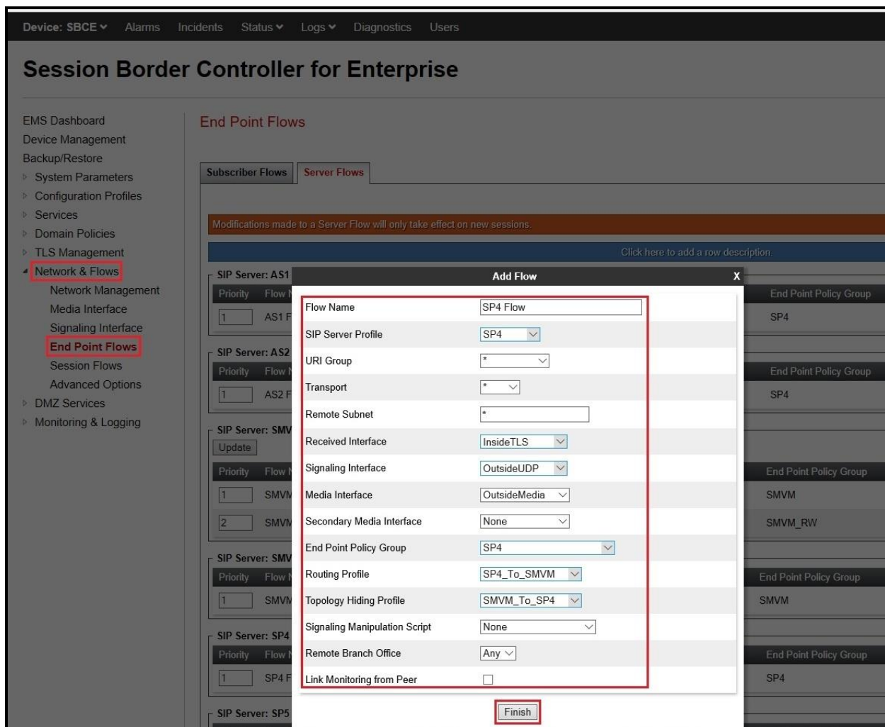
Figure 83: End Point Flow 2
