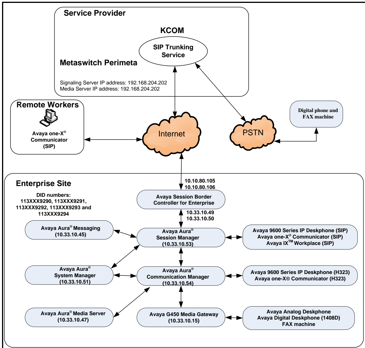
Figure 1: Avaya IP Telephony Network and KCOM SIP Trunk
