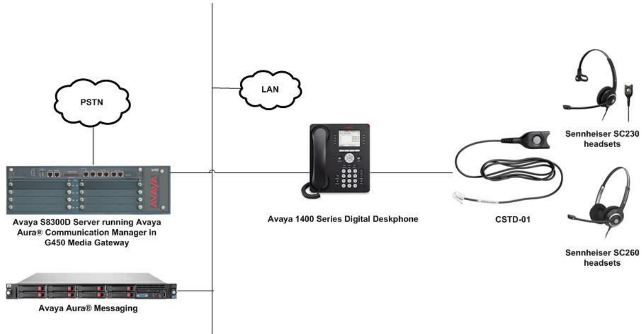
Figure 1: Avaya 1400 Series Digital Deskphones with Sennheiser SC 230 /SC 260 Headsets
