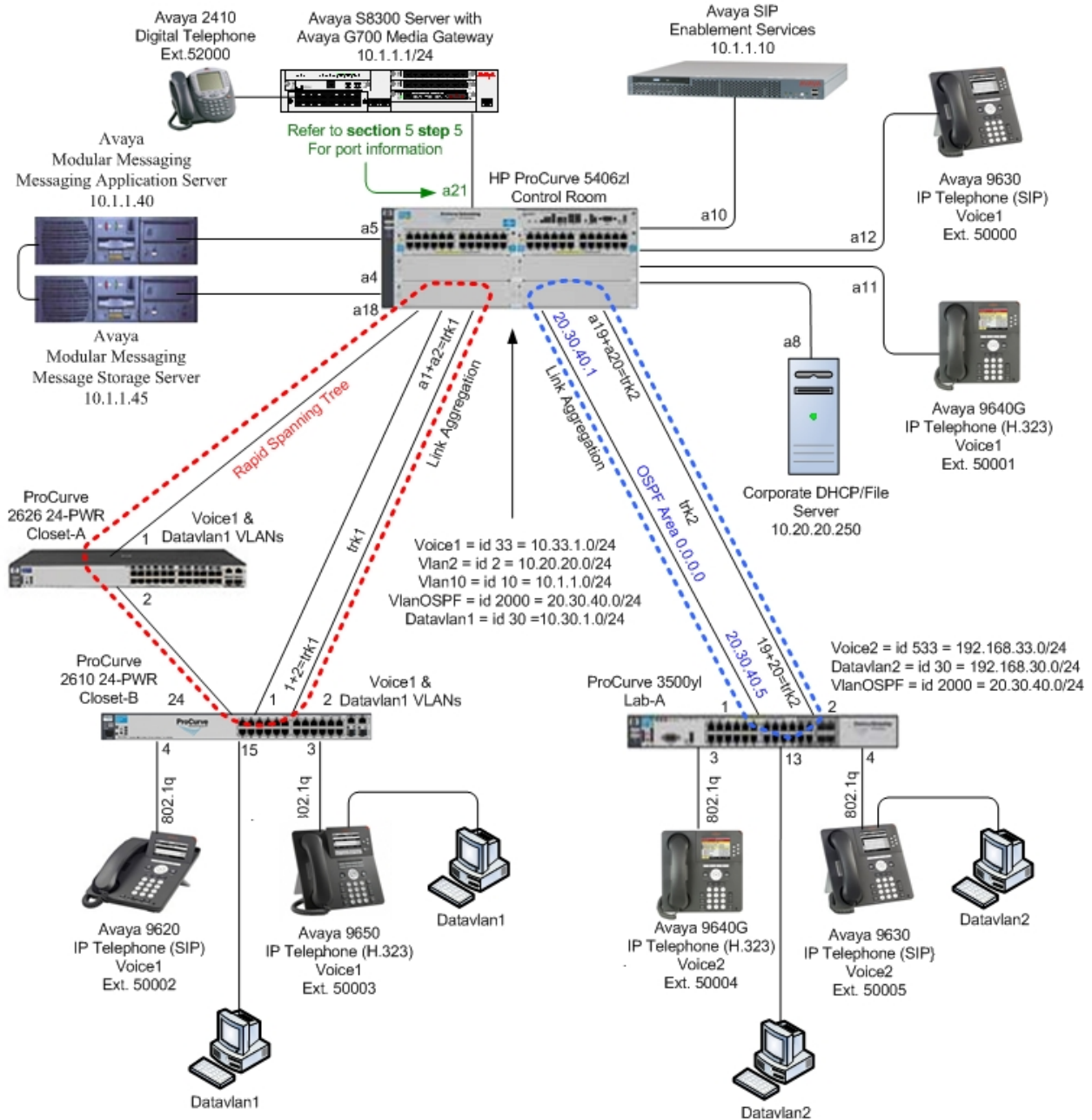
Figure 1: Network Configuration
