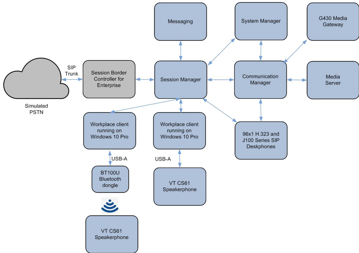
Figure 1: Test Configuration
