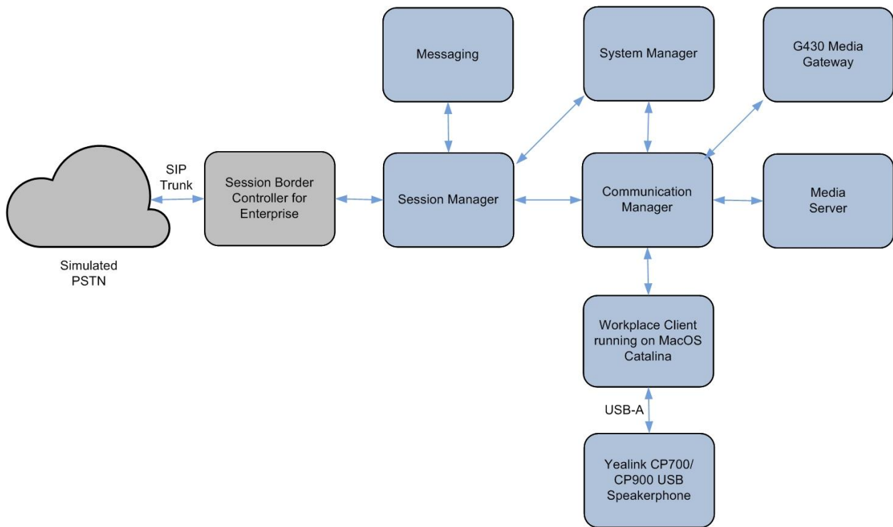
Figure 1: Test Configuration
