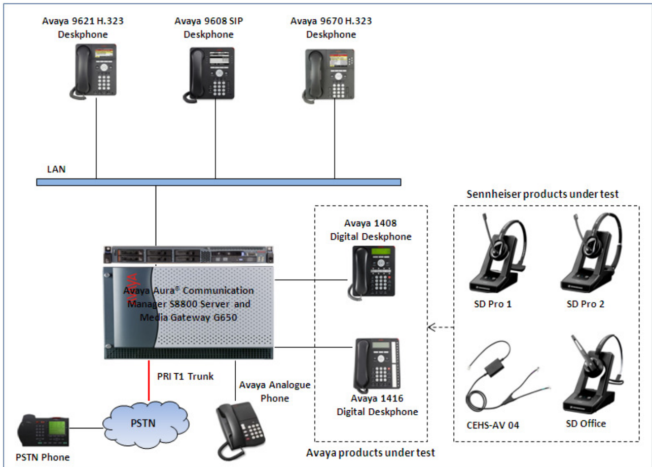
Figure 1: Test diagram for Avaya 1400 Series Digital Deskphone with Sennheiser Communications A/S CEHS-AV 04 EHS Adapter and SD Pro1, SD Pro2 and SD Office Wireless Headsets.
