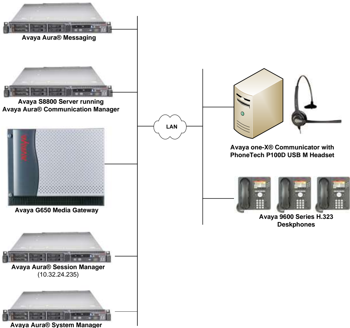
Figure 1: Avaya one-X® Communicator with PhoneTech P100D USB M Headset
