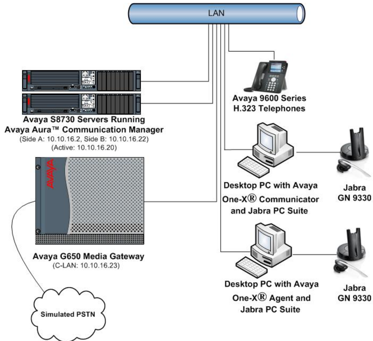
Figure 1: Network Topology
