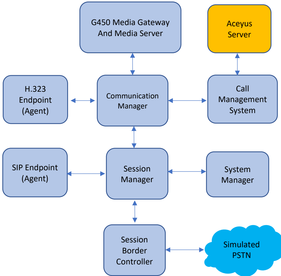
Figure 1: Network Configuration
