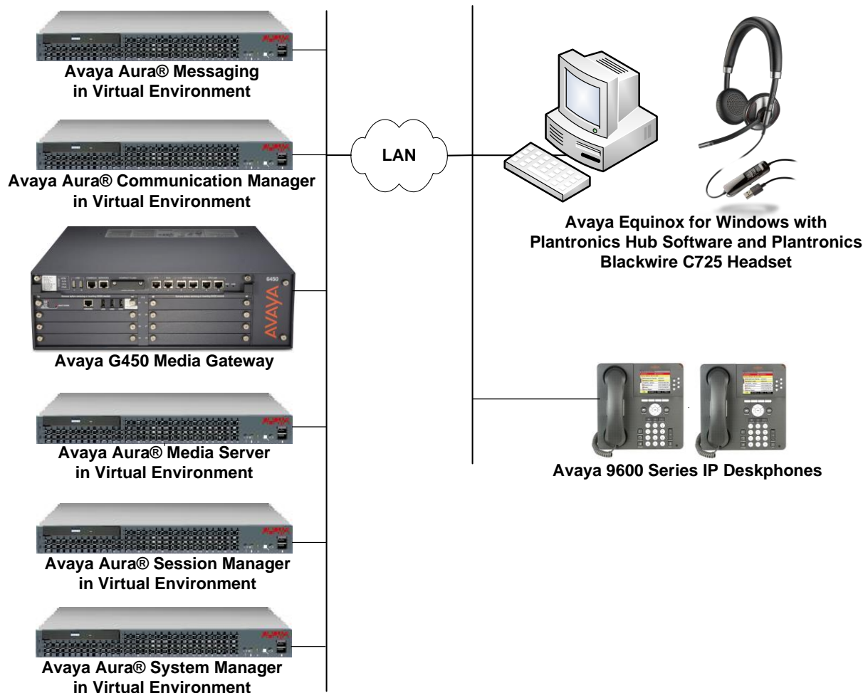
Figure 1: Avaya Equinox for Windows with Plantronics Hub Software and Plantronics Blackwire C725 Headset
