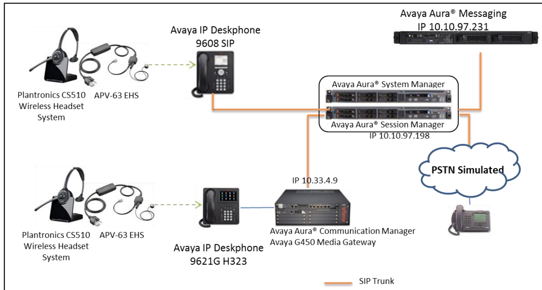
Figure 1: Avaya 96x1 Series IP Deskphones with Plantronics APV-63 EHS Adapter and Plantronics CS510 Wireless Headset System
