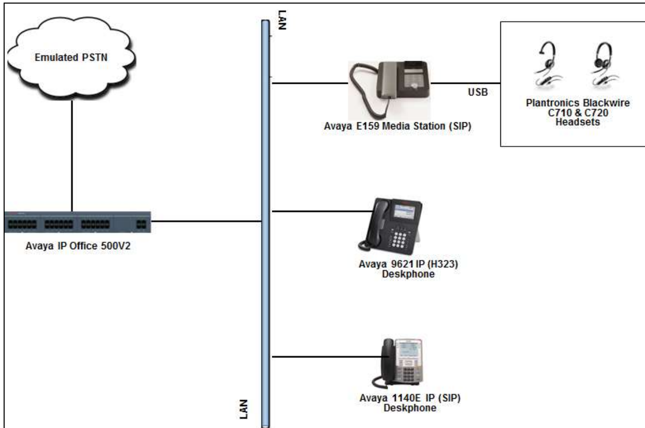
Figure 1: Test Configuration
