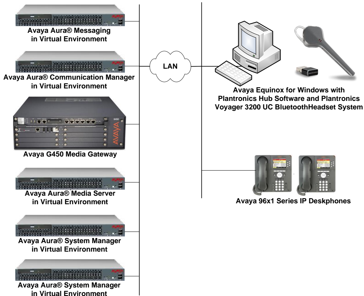
Figure 1: Avaya Equinox with Plantronics Hub Software and Plantronics Voyager 3200 UC Bluetooth Headset System
