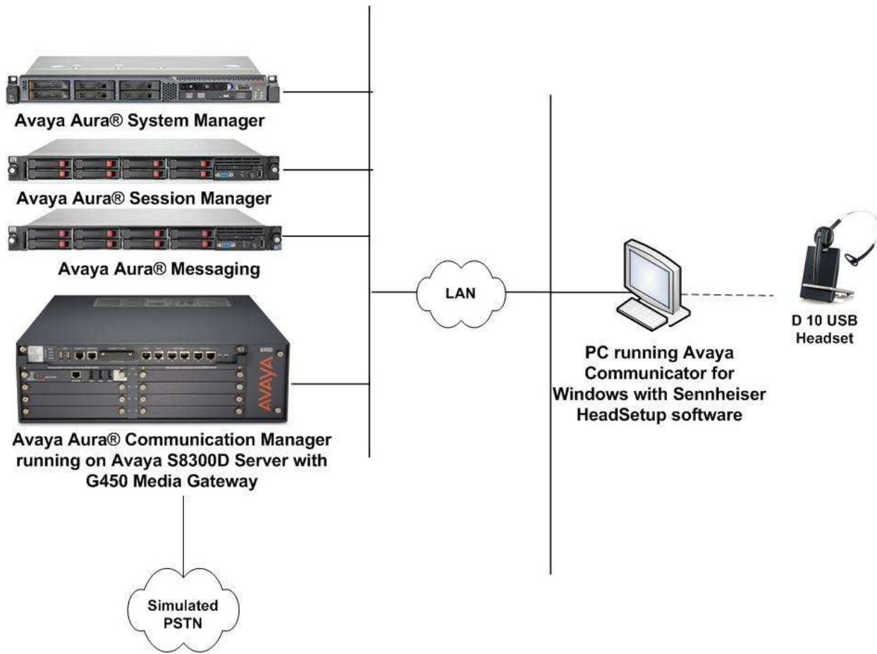
Figure 1: Test Configuration
