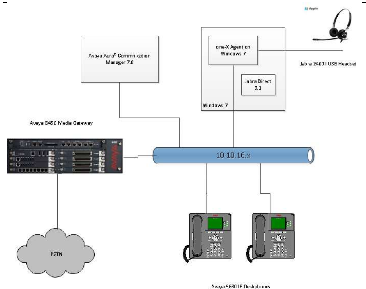
Figure 1: Avaya one-X Agent with Jabra BIZ 2400 II USB Headsets
