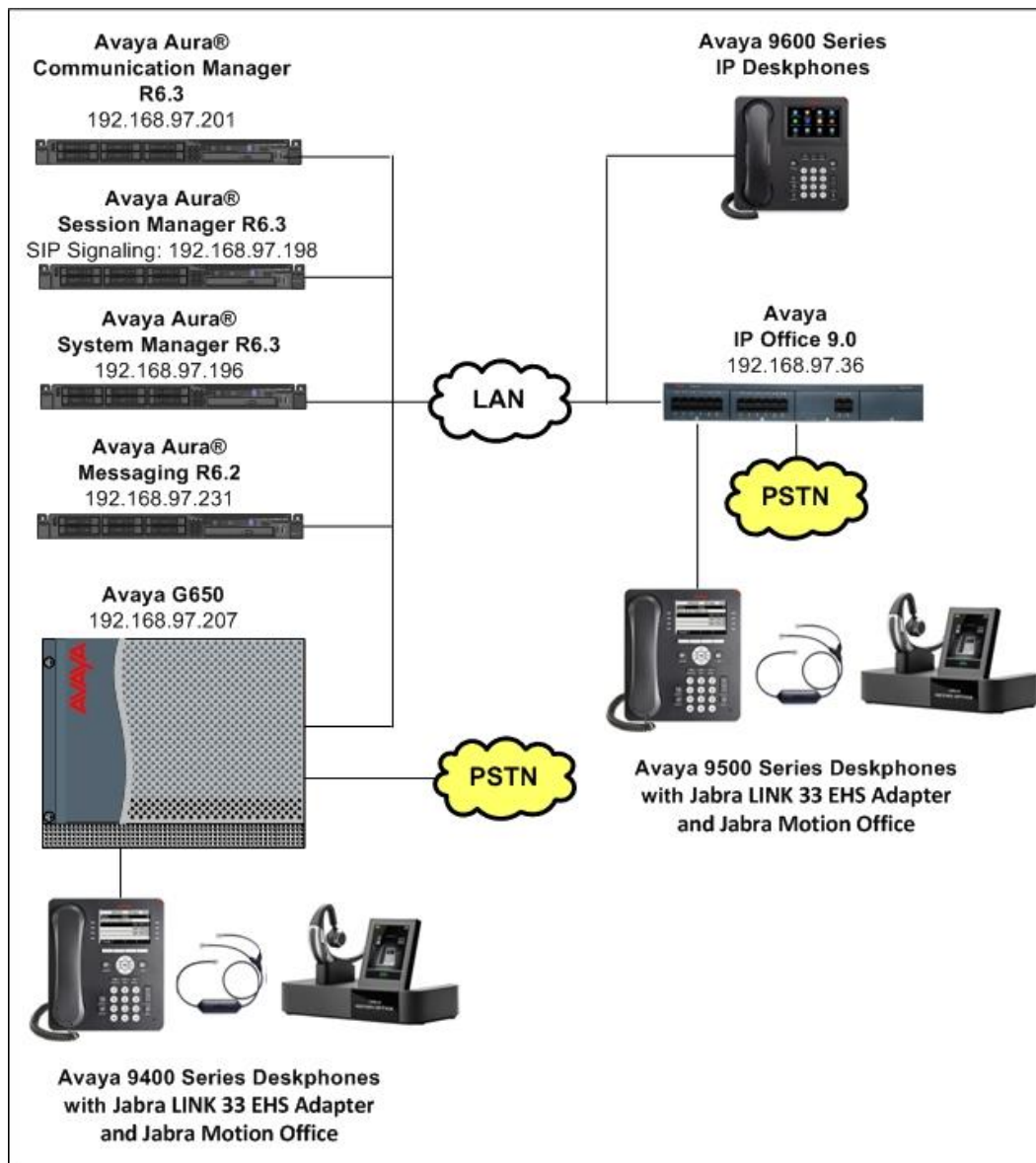
Figure 1: Avaya 9400/9500 Series Digital Deskphones with Jabra LINK 33 EHS Adapter and Jabra Motion Office
