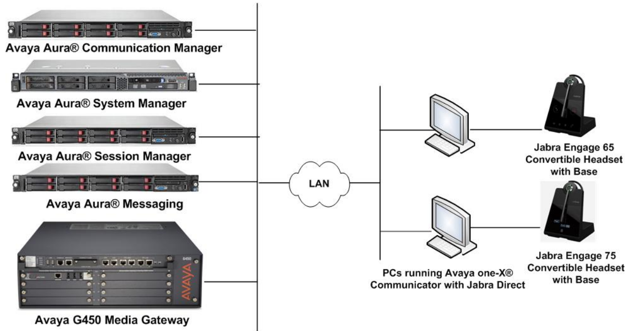
Figure 1: Test Configuration
