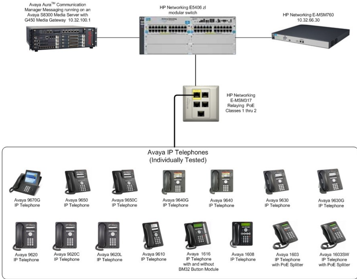
Figure 1: HP Networking E-MSM317 MultiService Access Device & Avaya IP Telephones
