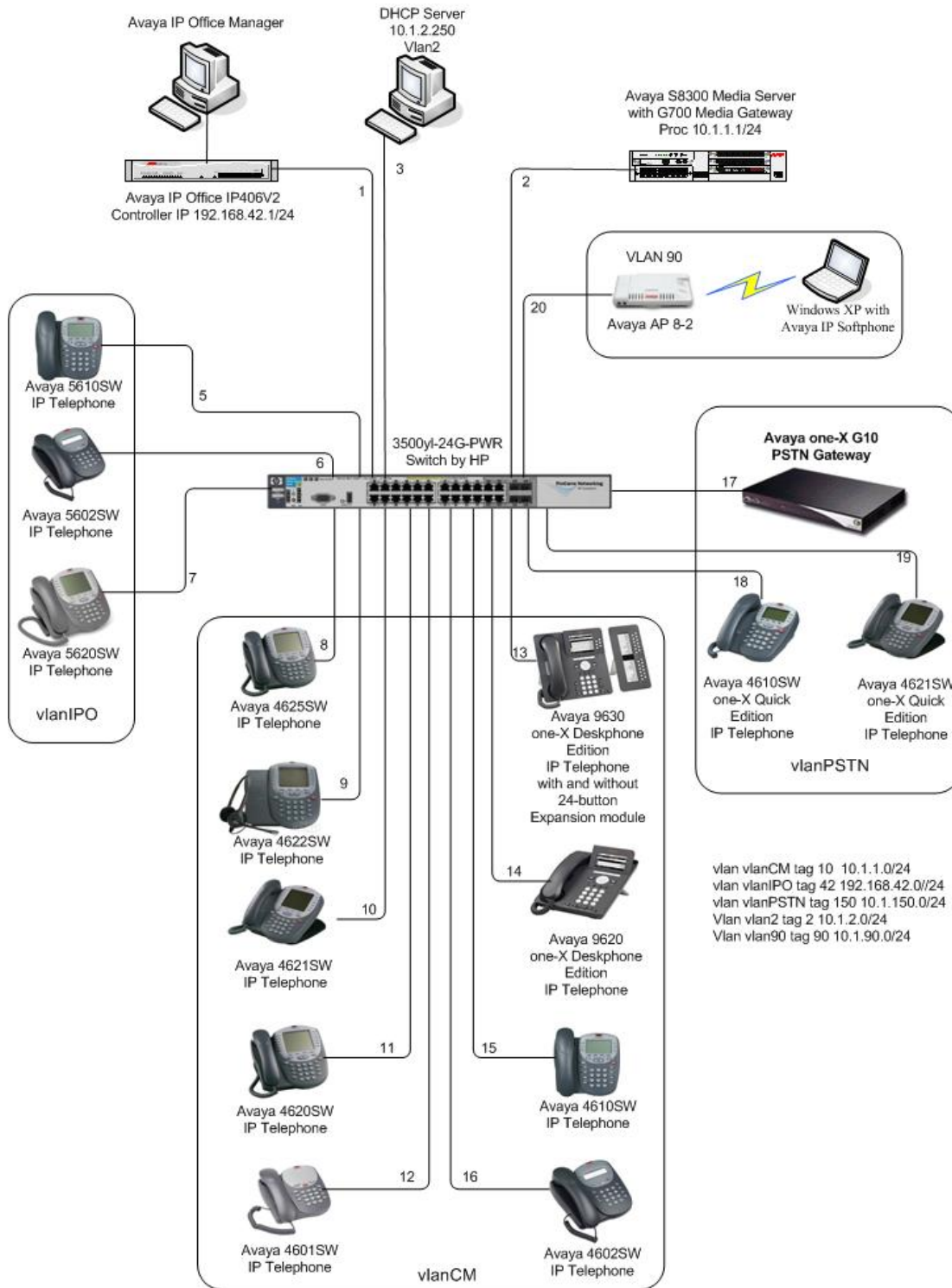
Figure 1: PoE Interoperability between 3500yl-24G-PWR, Avaya IP Telephones and Avaya one-X Quick Edition G10 PSTN Gateway
