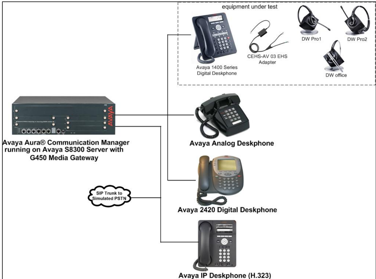
Figure 1: Avaya 1400 Series Digital Deskphone with Sennheiser Communications A/S CEHS-AV 03 EHS Adapter and DW Pro1, DW Pro2, DW Office Wireless Headsets.
