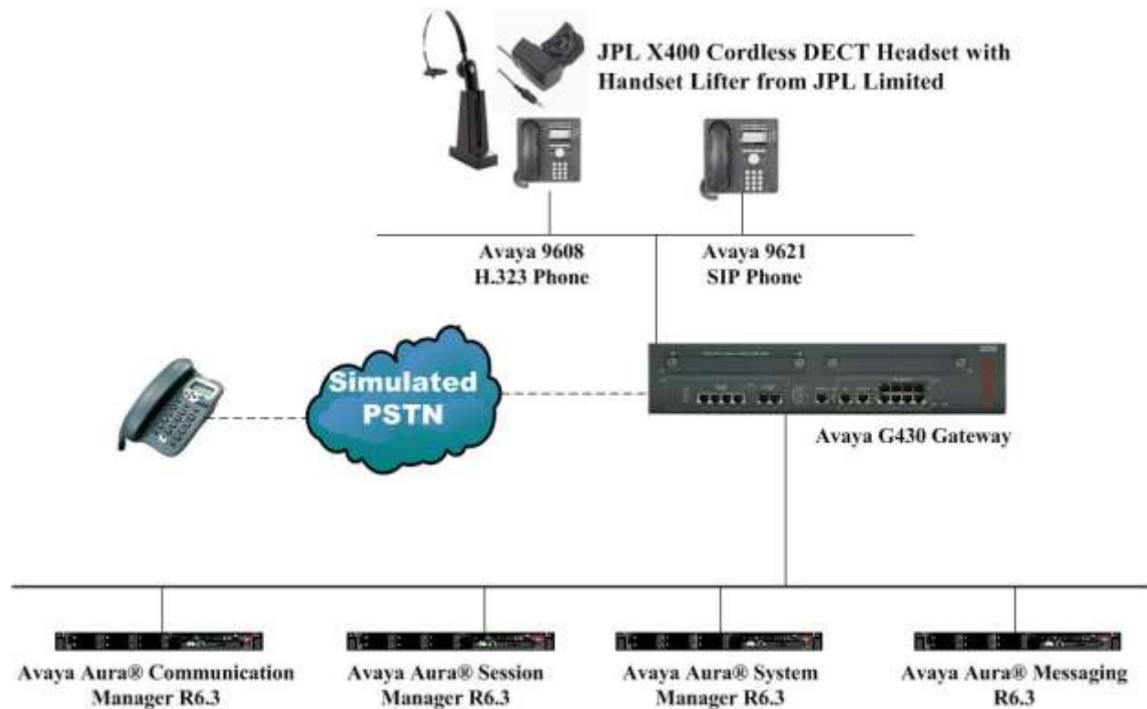
Figure 1: Network Solution of the JPL X400 Cordless DECT Headset with Handset Lifter connecting to Avaya 96x1 Series IP Telephones
