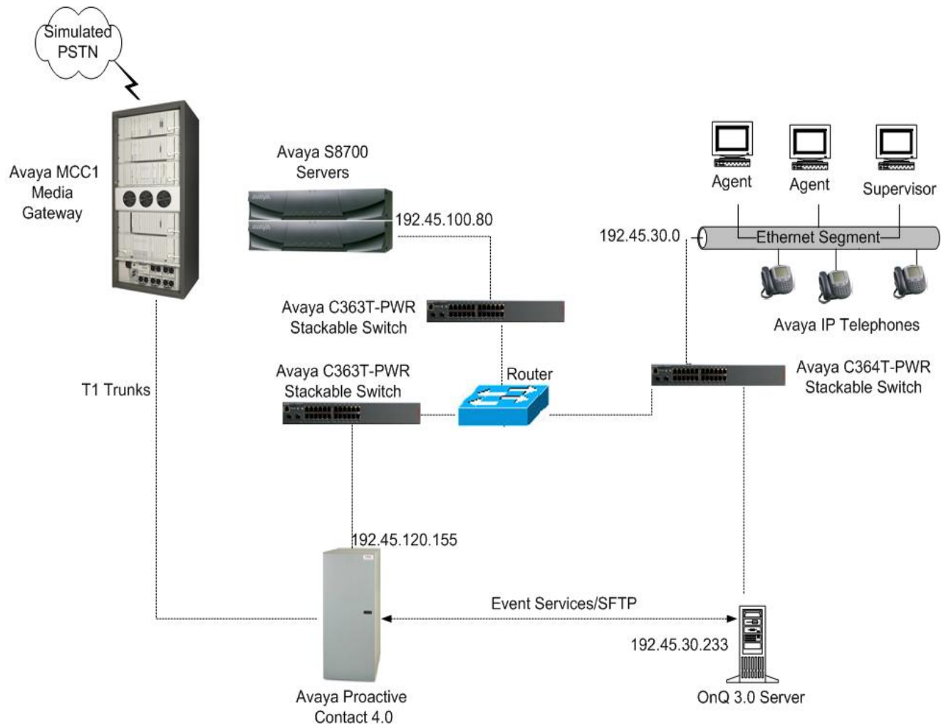
Figure 1: Avaya Proactive Contact 4.0 and Austin Logistics OnQ 3.0 Integration
