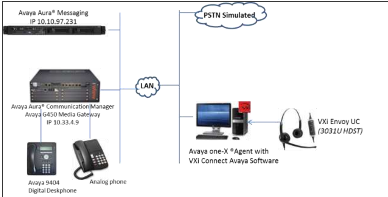
Figure 1: Test configuration Avaya one-X® Agent with VXi Connect Avaya and VXi Headsets
