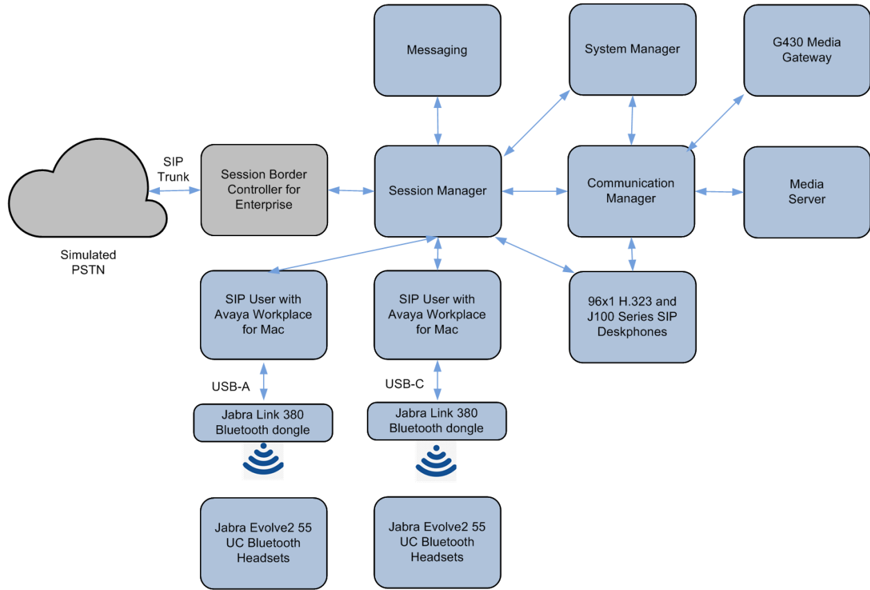
Figure 1: Test Configuration
