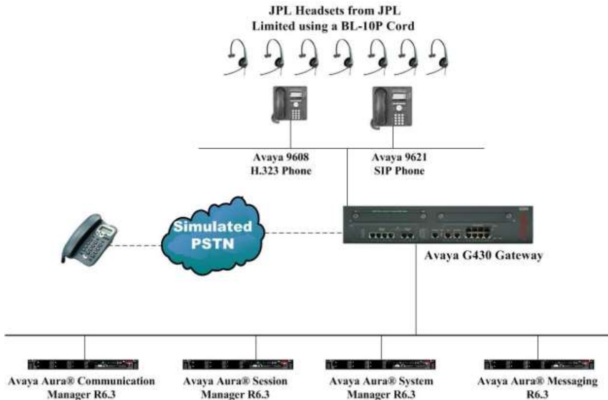
Figure 1: Network Solution of the JPL Headsets connecting to Avaya 96x1 Series IP Telephones using a BL-10P cord
