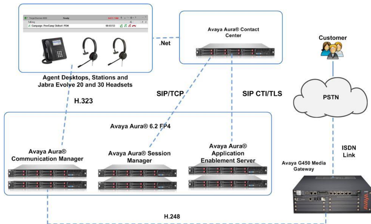
Figure 1: Test Configurations
