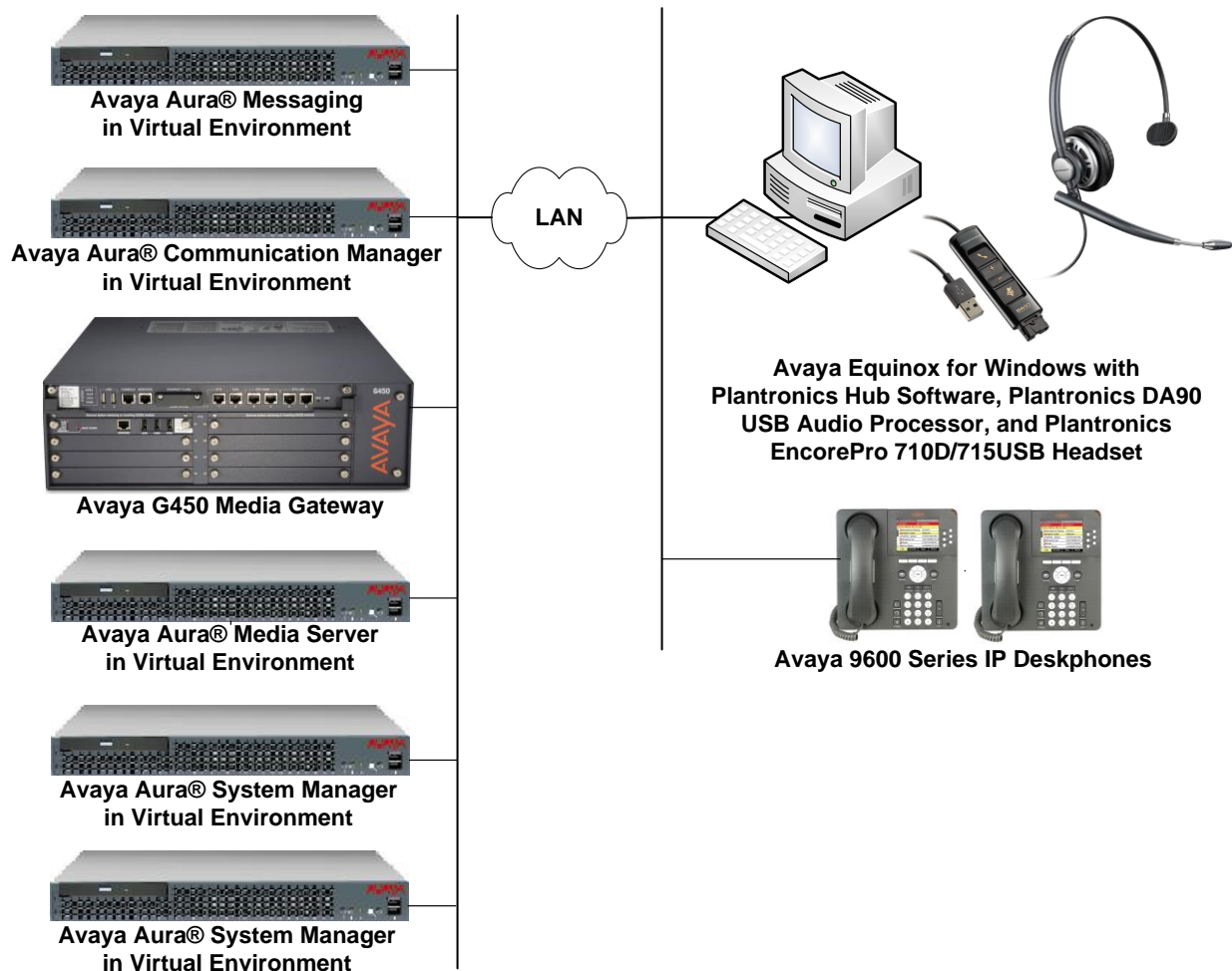
Figure 1: Avaya Equinox for Windows with Plantronics Hub Software, Plantronics DA90 USB Audio Processor, and Plantronics EncorePro 710D/715USB Headset
