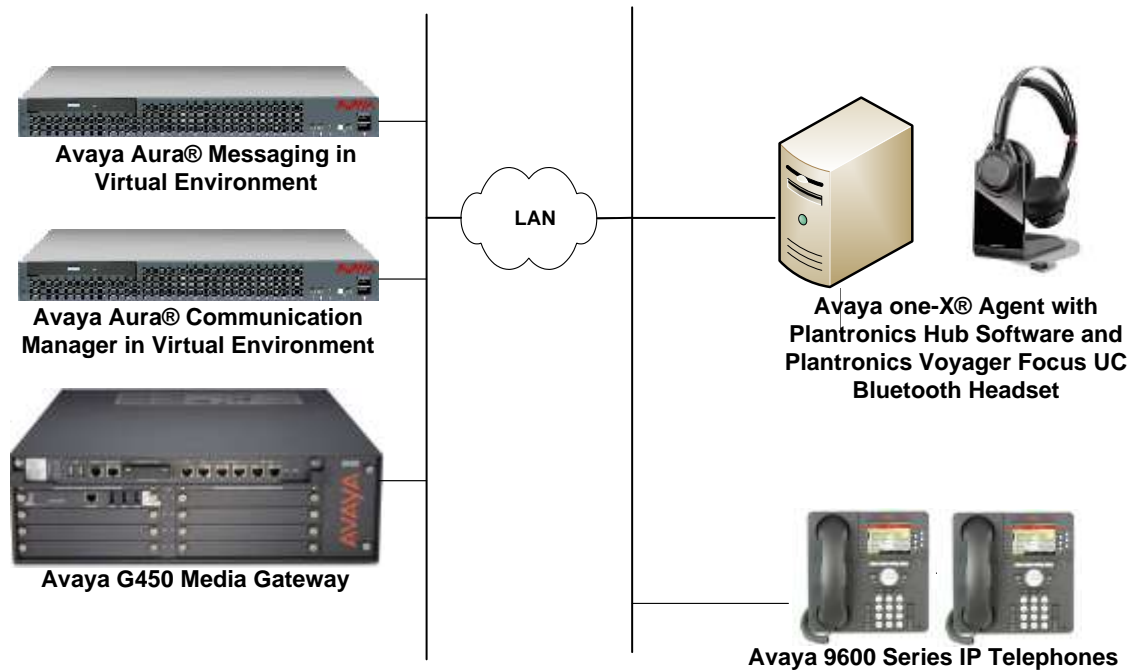
Figure 1: Avaya one-X Agent with Plantronics Hub Software and Plantronics Voyager Focus UC Bluetooth Headset
