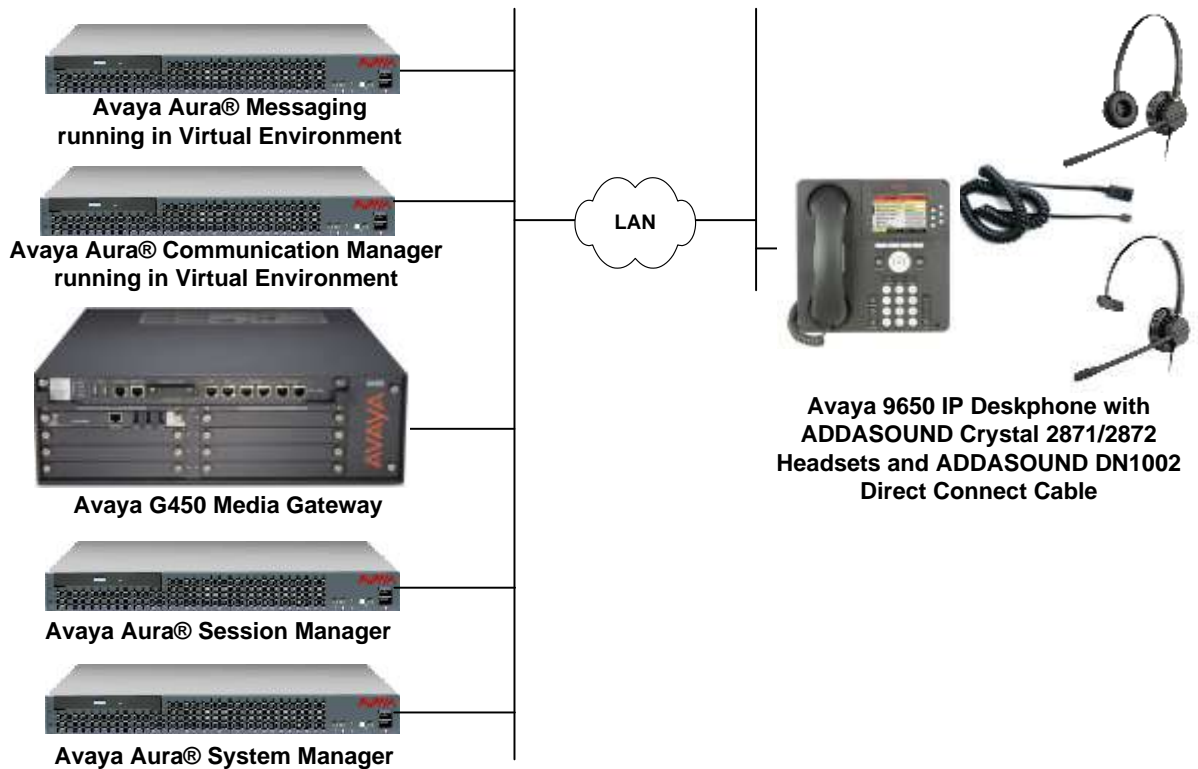
Figure 1: Avaya 9600 Series IP Telephone with ADDASOUND Crystal 2871/2872 Headsets and DN1002 Direct Connect Cable
