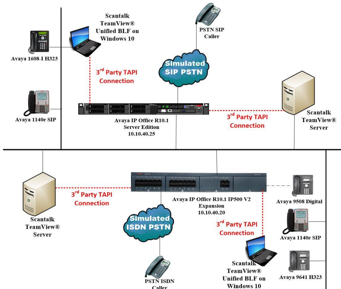
Figure 1: Scantalk TeamView® Unified BLF with Avaya IP Office Server Edition and Server Edition Expansion IP500 V2
