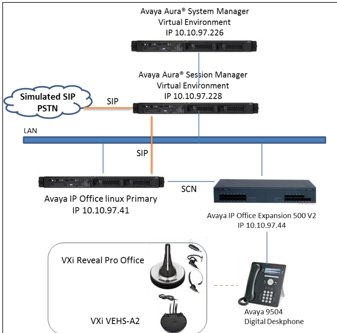
Figure 1: Test diagram for Avaya 9500 Series Digital Deskphone with VXi Reveal Pro Office Headsets and VXi VEHS-A2 EHS Cable.
