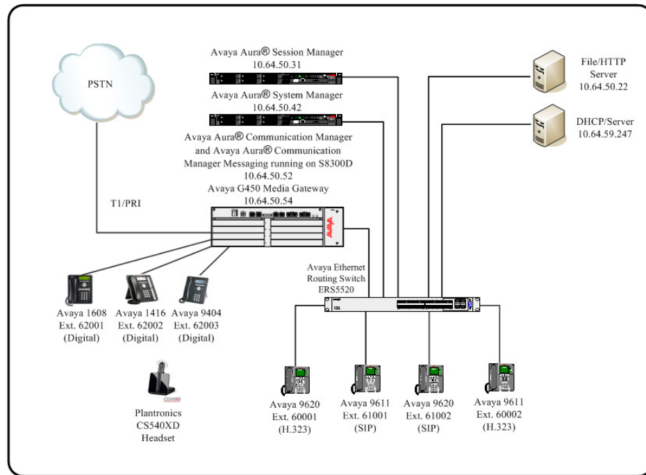
Figure 1: Avaya 1400 Series Digital Telephone with Plantronics APV-63 EHS Adapter and Plantronics CS540XD Wireless Headset System
