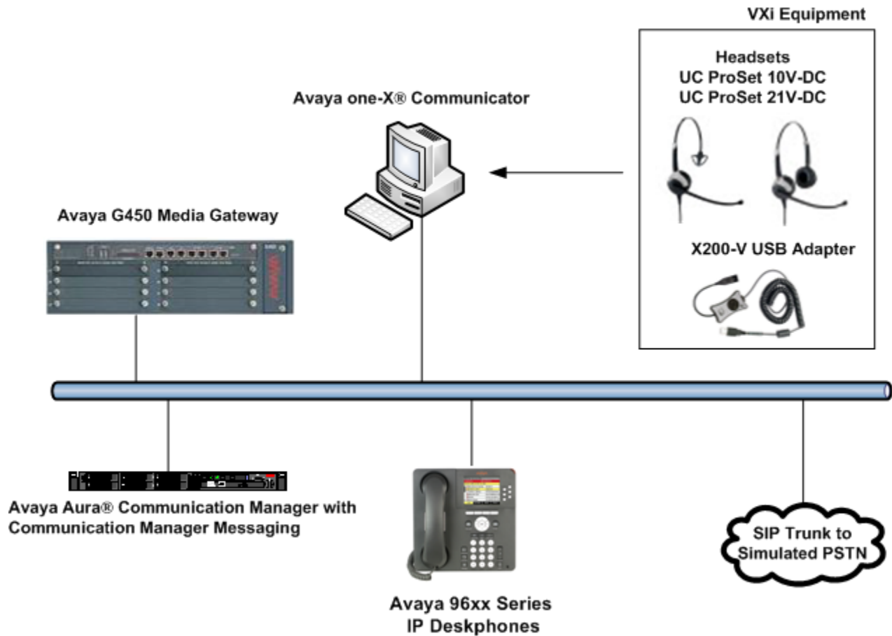
Figure 1: Test Configuration
