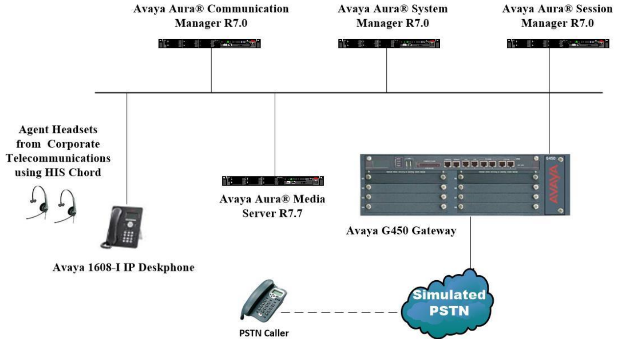
Figure 1: Network Solution of the Corporate Telecommunications Agent Headsets connecting to Avaya 1600 Series IP Telephones using a HIS chord
