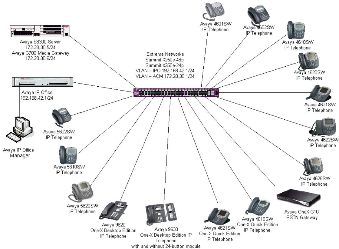
Figure 1: PoE sample network configuration
