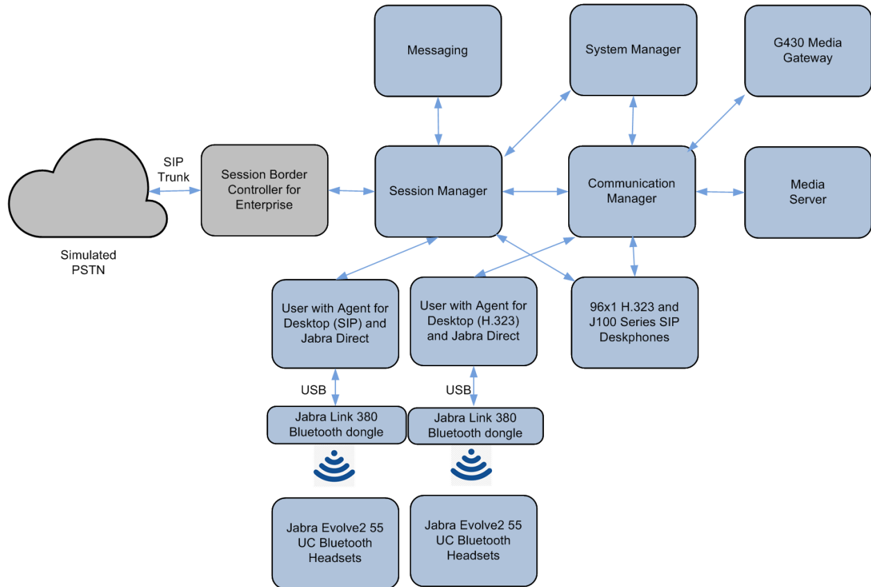
Figure 1: Test Configuration
