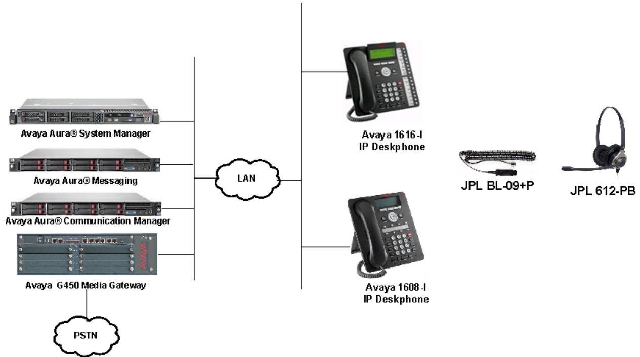
Figure 1: Test Configuration
