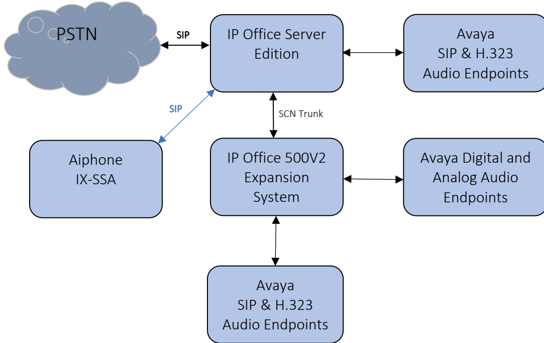
Figure 1: Test Configuration of Aiphone IX-SSA with Avaya IP Office
