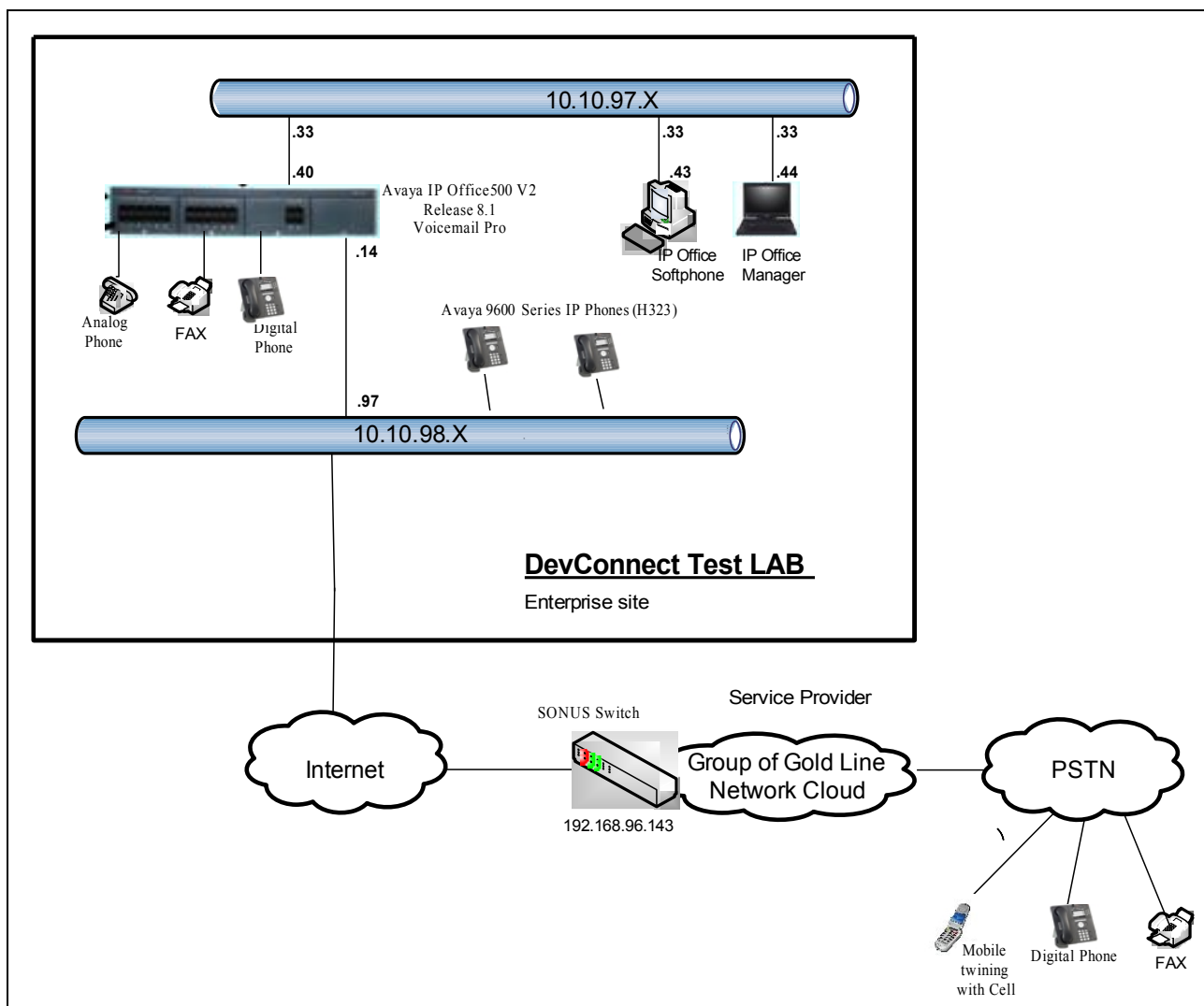
Figure 1: Test Configuration for Avaya IP Office with Group of Gold Line Inc SIP Trunking Service
