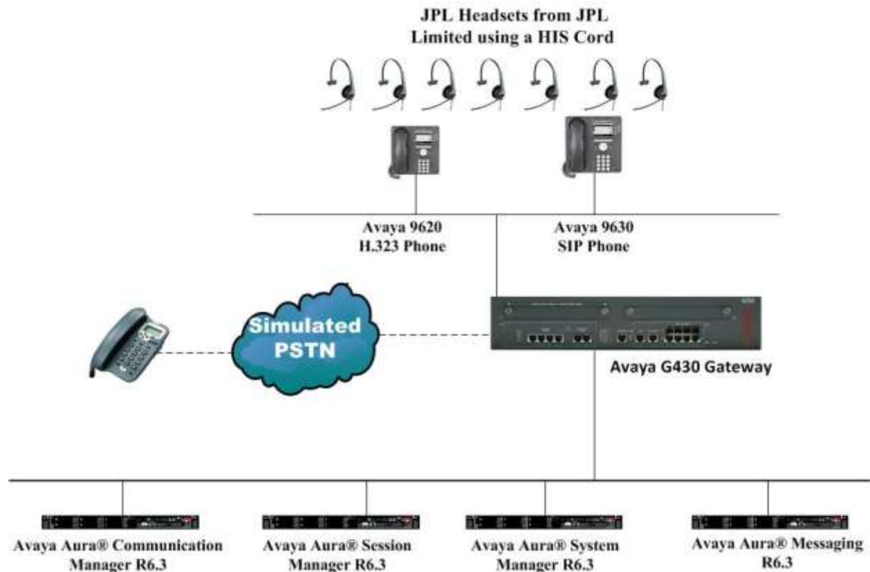
Figure 1: Network Solution of the JPL Headsets connecting to Avaya 9600 Series IP Telephones using a HIS cord
